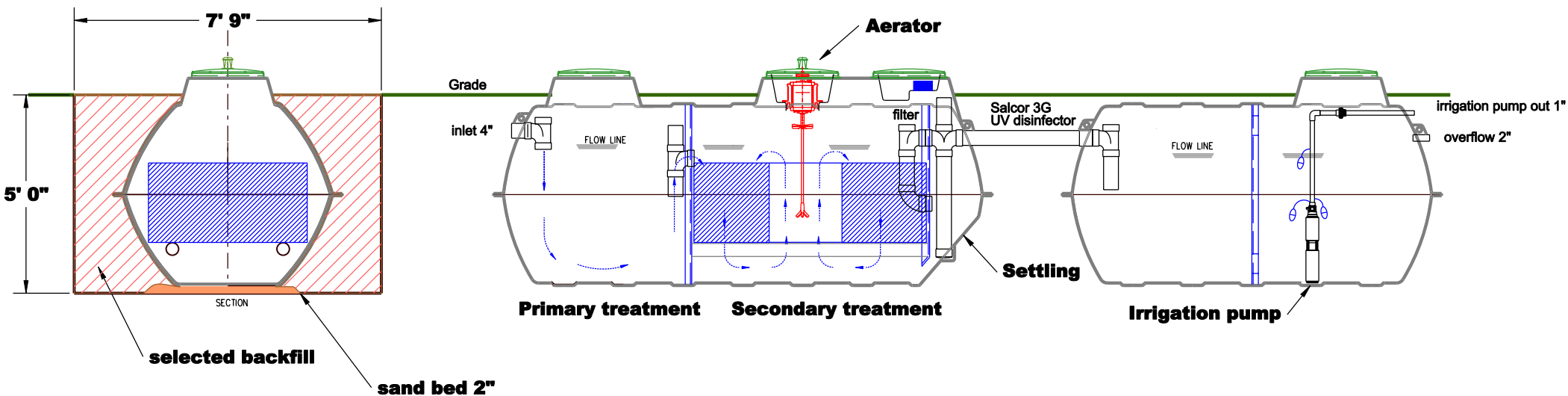
Typical section
